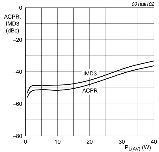
Fig 6. 2-carrier W-CDMA adjacent channel leakage ratio and IMD3 as functions of average load power; typical values
